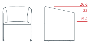
Lounge armchair on castors 1PL6021: L 22 D 22 \frac{3}{4} H 26 \frac{1}{2}
