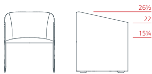
Lounge armchair on feet 1PL6022: L 22 D 22 \frac{3}{4} H 26 \frac{1}{2}
