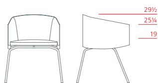
Armchair on four legs 1PL6030: L 25 \frac{1}{2} D 23 H 29 \frac{1}{2}
